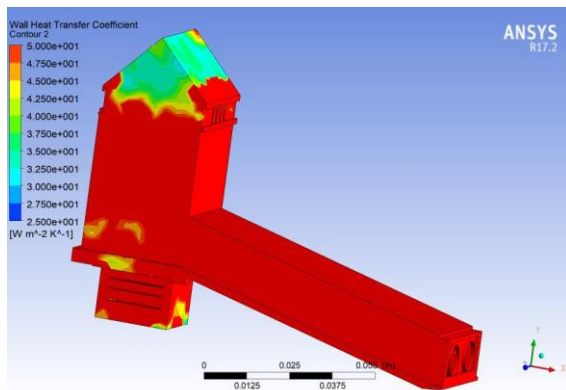
Figure 12: Wall heat transfer coefficient of the drying system
