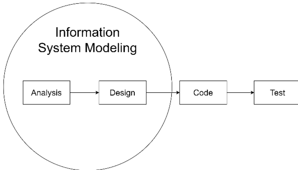
Fig. 1. Waterfall Model
