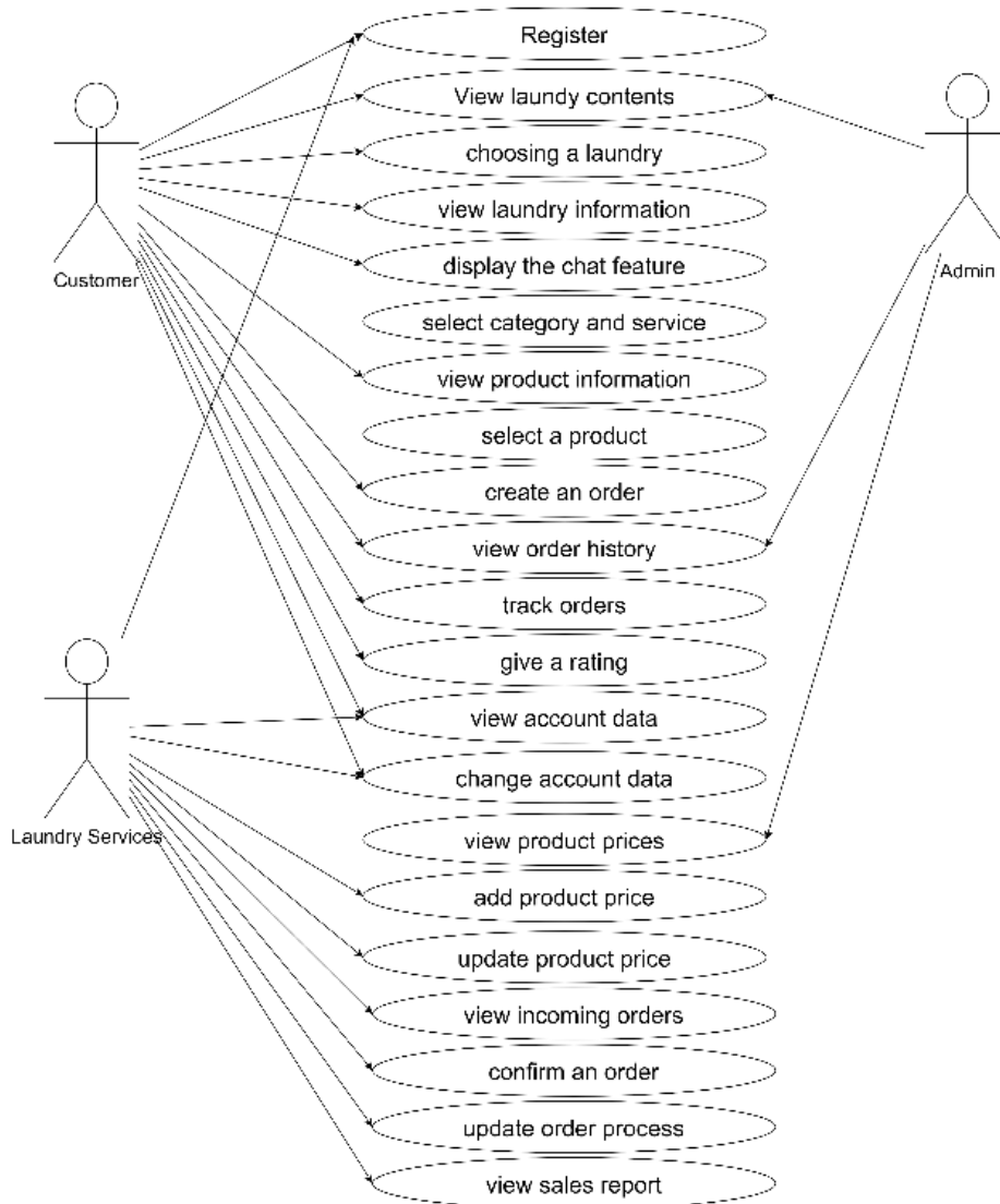
Fig. 2. Use Case Diagram
